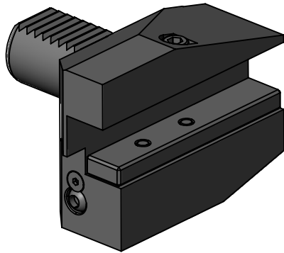
90DEG VDI30 STATIC TOOL OUTPUT: 3/4 SQR SHANK COOLANT: EXTERNAL
